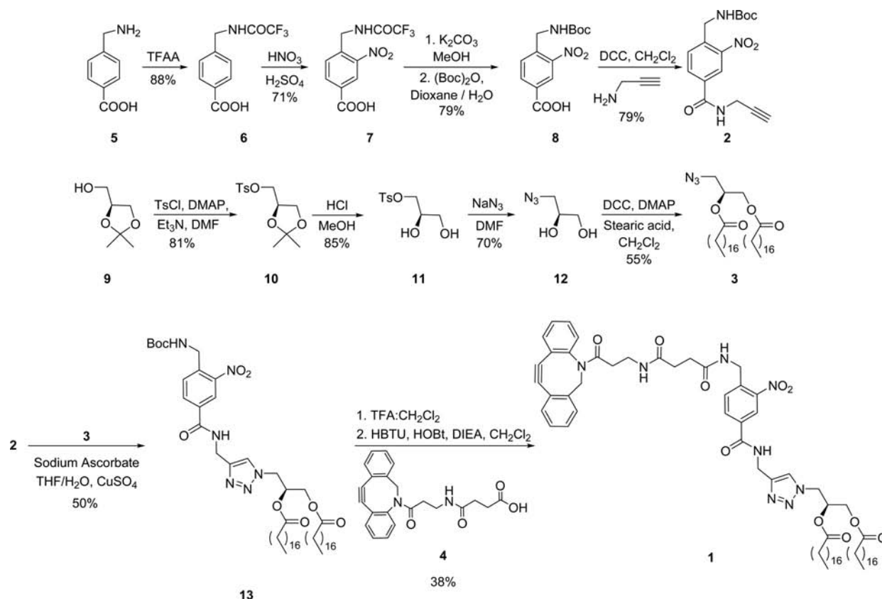
Scheme 1. Synthetic Route to Clickable and Photocleavable Lipid Delivery Agent 1
